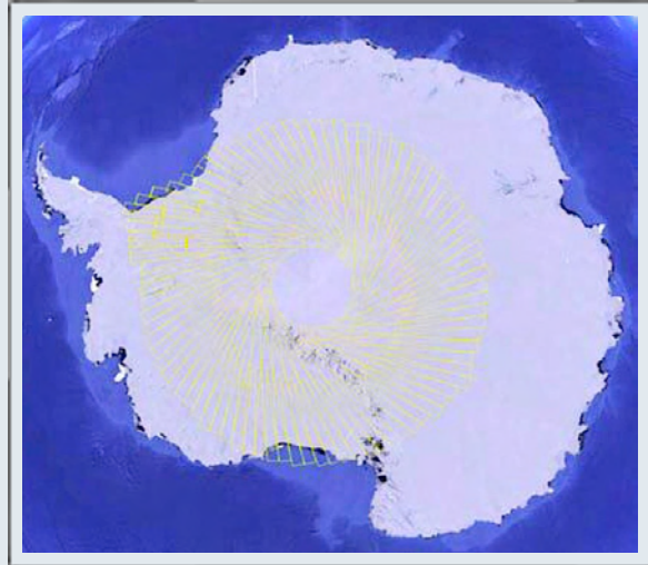
RADARSAT-2 SAR S5 coverage plan for parts of Antarctica, the plan is currently under consideration and may be spread over multiple years]
