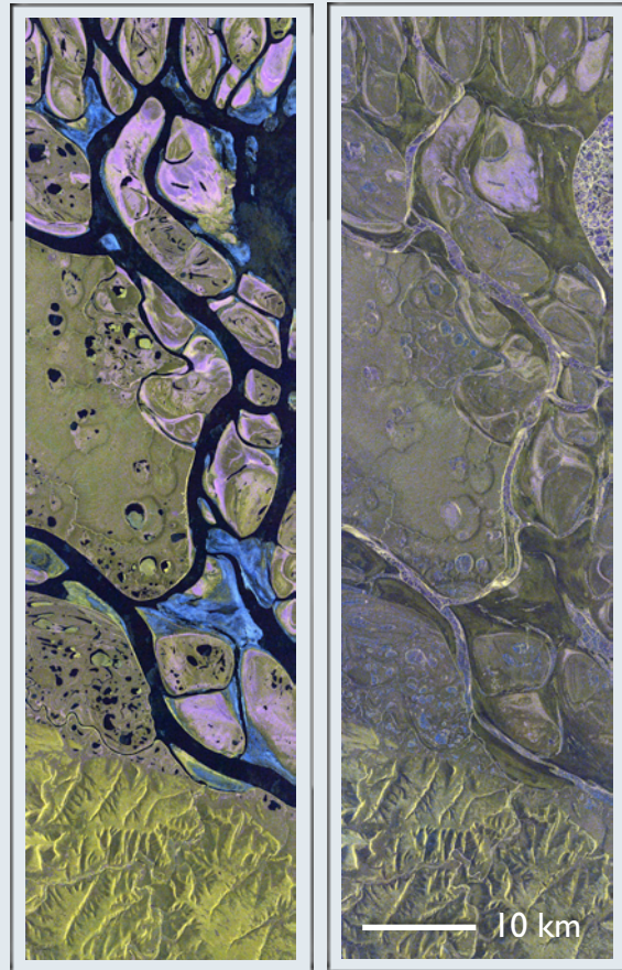
TerraSAR-X image products in HH/HV polarization acquired over the Kytalyk / Lena Delta region in Russia on July 6, 2015 (left, open water conditions) and on October 24, 2015 (right, frozen).
